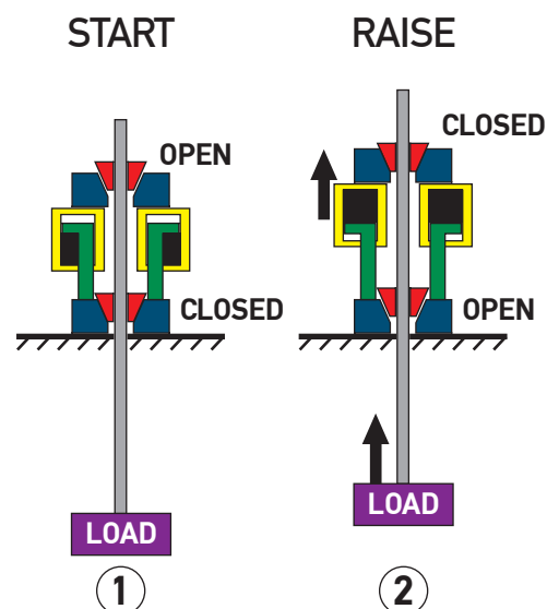
FIGURE 3 Operating sequence for strand jacks
