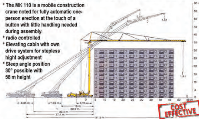
Liebherr MK 110, year 07/2006, maximum capacity 8 t/14 m, maximum radius 52 m/1,8 t
