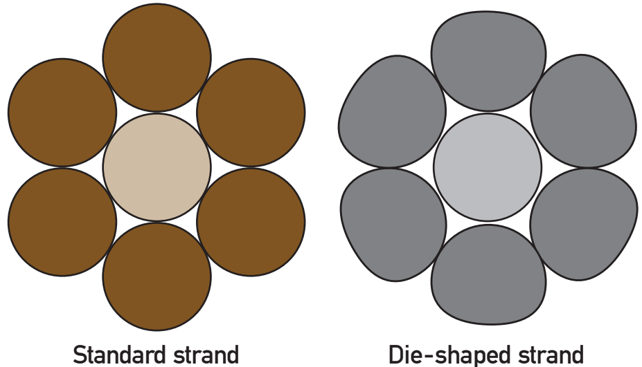
FIGURE 2 Standard strand on the left and a die-formed strand for strand jacking
